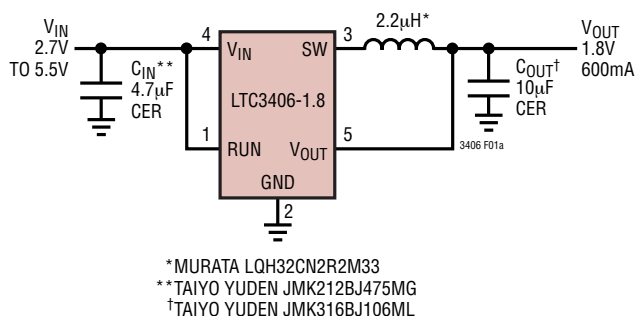
Figure 1a. High Efficiency Step-Down Converter
