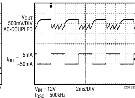
VOUT Transient (Burst Mode Operation, MODE = H)
