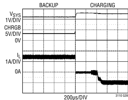
Backup to Charge Transient in Autonomous Application
