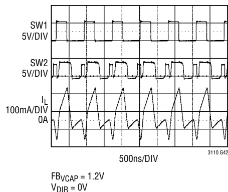
PWM Mode Operation in V_{CAP} Overvoltage Failure Condition
