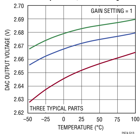
DAC Full-Scale Voltage vs Temperature, Gain Setting = 1
