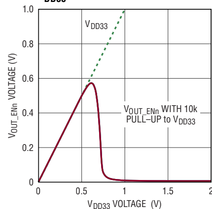
V_{OUT\_EN[3:0]} Output Voltage vs V_{DD33}
