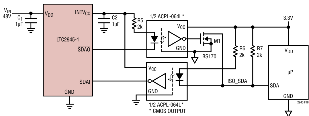
Figure 18. Opto-Isolation of I²C Interface with Low Power, High Speed Opto-Couplers (SCL Omitted for Clarity)
