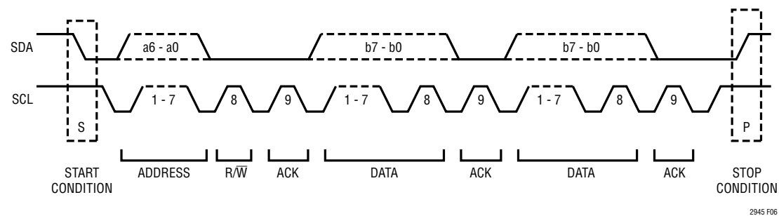
Figure 6. General Data Transfer Over I²C
