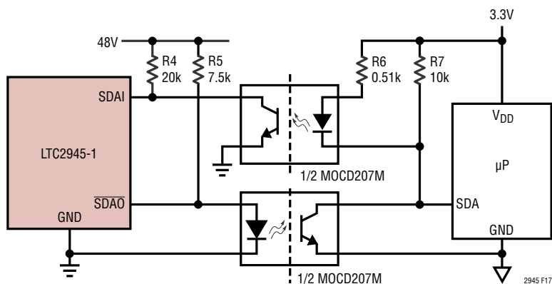
Figure 17. Opto-Isolation of a 1.5kHz I²C Interface Between LTC2945-1 and Microcontroller (SCL Omitted for Clarity)
