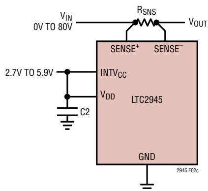
(c) Power from Low Voltage Secondary Supply Figure 2. LTC2945 Derives Power
