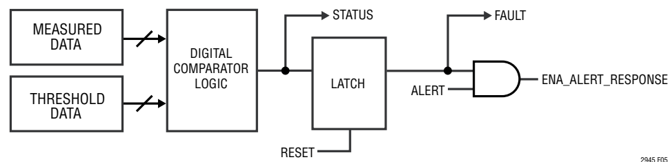
Figure 5. LTC2945 Fault Alert Generation Blocks
