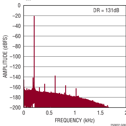
128k Point FFT f_{SAMPL} = 1\text{Mps} , f_{IN} = 200\text{Hz} , DF = 256
