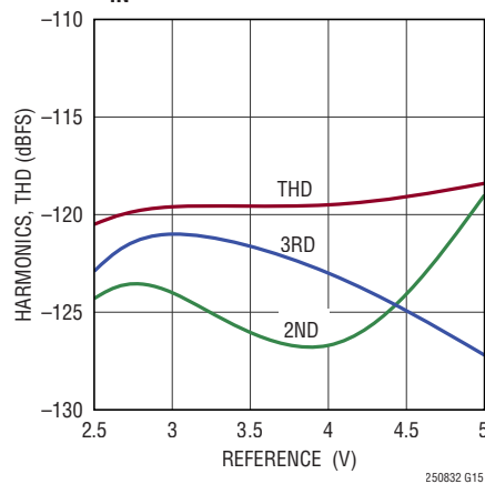
THD, Harmonics vs Reference Voltage, f_{IN} = 200\text{Hz} , A_{IN} = -1\text{dBFS}
