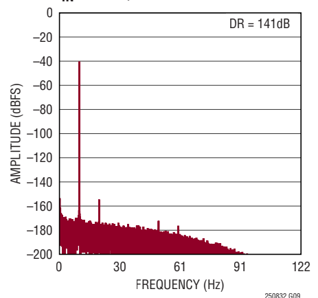
32k Point FFT f_{SAMPL} = 1\text{Mps} , f_{IN} = 10\text{Hz} , DF = 4096
