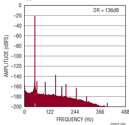
128k Point FFT f_{SAMPL} = 1\text{Mps} , f_{IN} = 50\text{Hz} , DF = 1024
