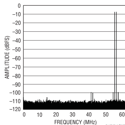
64k Point 2-Tone FFT, f_{IN} = 69MHz , 70MHz, -1dBFS , 125Mps
