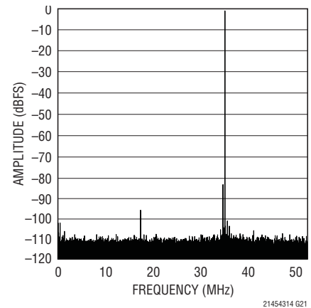
LTC2144-14: 64k Point FFT, f_{IN} = 140\text{MHz} , -1\text{dBFS} , 105Mps
