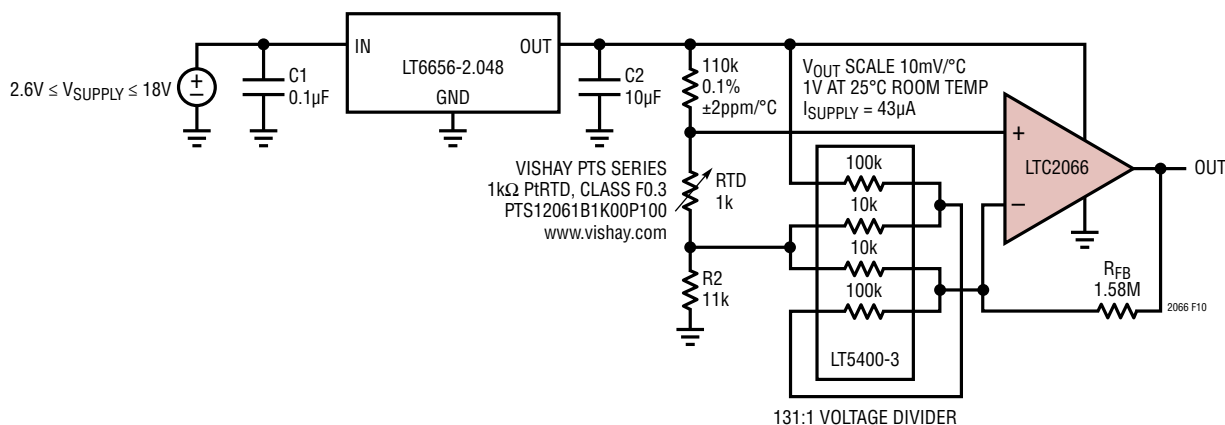
Figure 10. RTD Sensor
