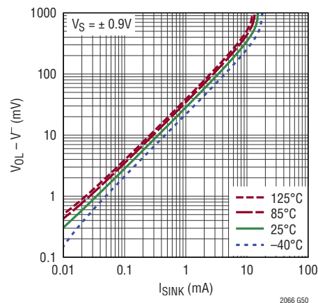
Output Voltage Swing Low vs Load Current
