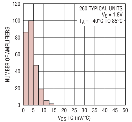
Input Offset Voltage Drift Distribution (I-Grade)
