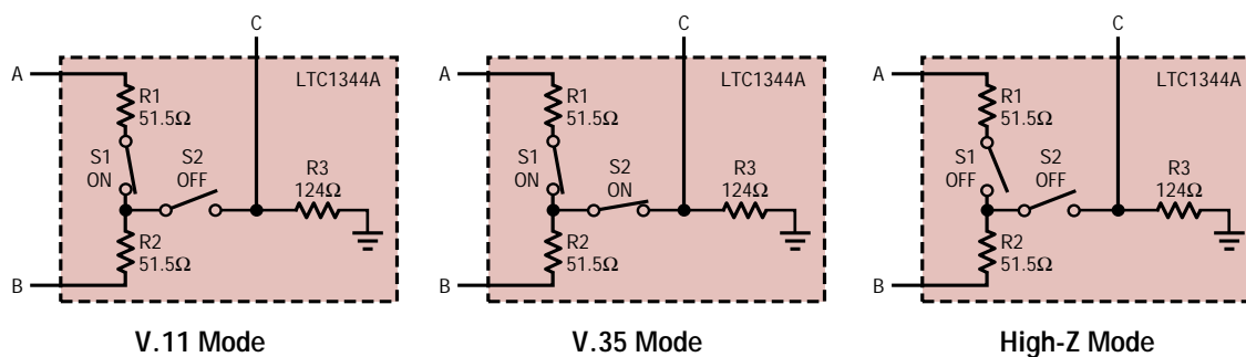
Figure 3. LTC1344A Modes
