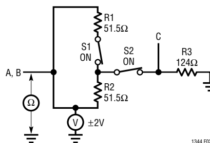
Figure 2. V.35 Common Mode Impedance Measurement
