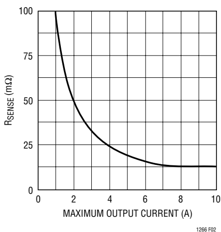
Figure 2. Selecting R_{SENSE}
