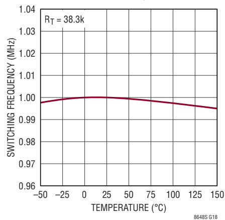
Switching Frequency
