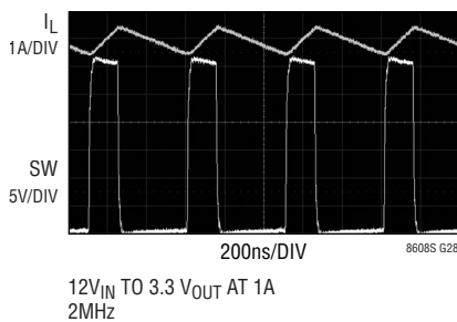
Switching Waveforms
