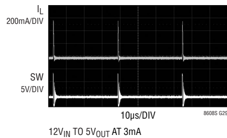
Switching Waveforms
