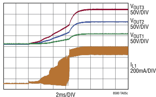
Start-Up Waveforms
