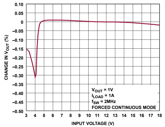
Figure 19. Line Regulation
