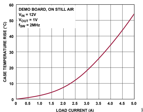
Figure 43. LT83203/LT83205 Case Temperature Rise
