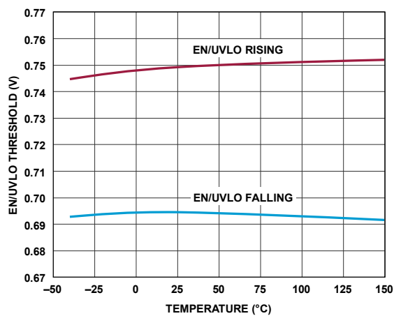
Figure 20. EN/UVLO Pin Thresholds
