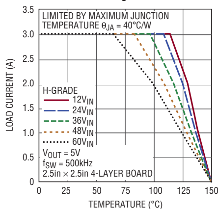
Thermal Derating
