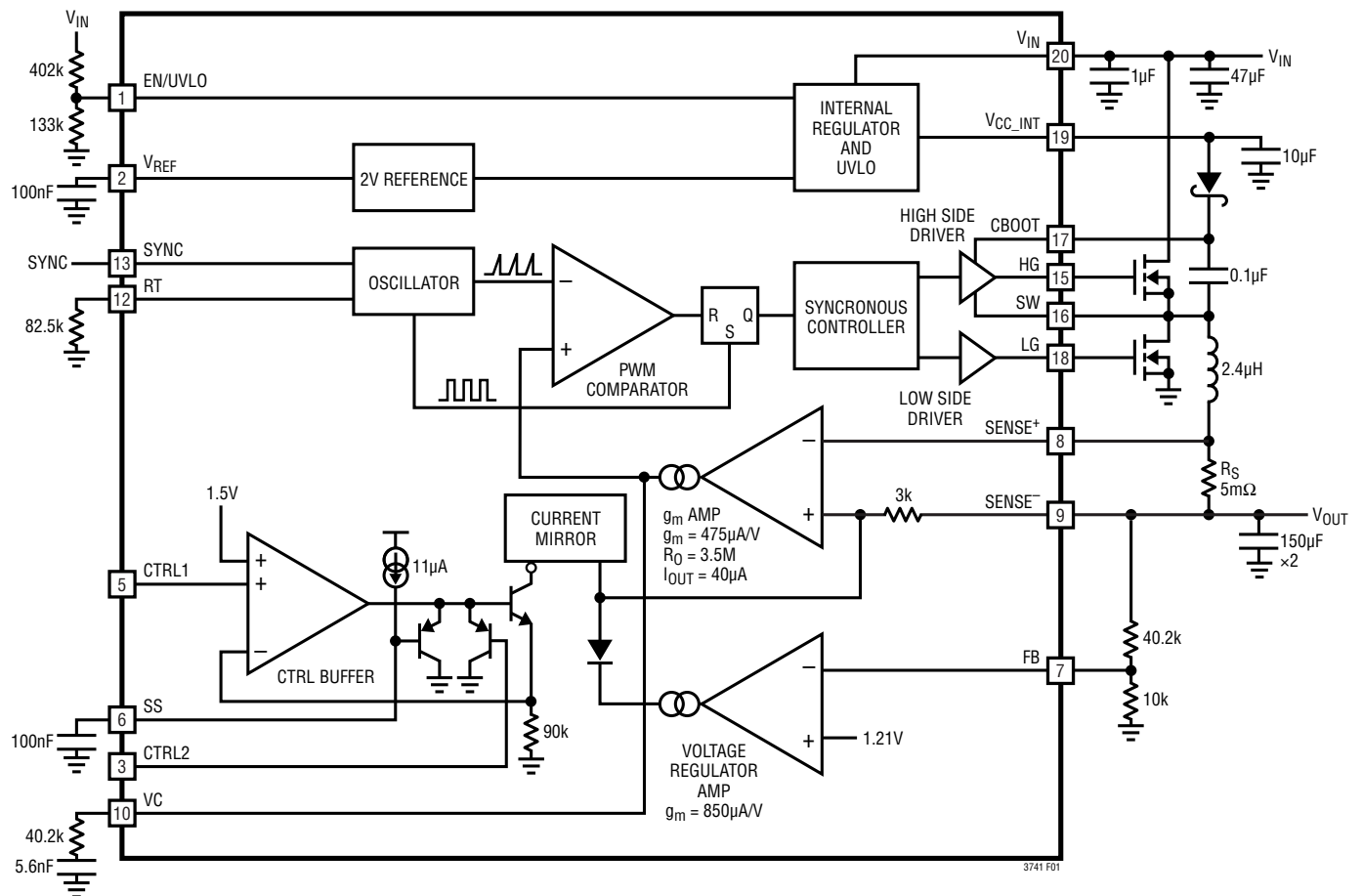
Figure 1. Block Diagram, LT3741
