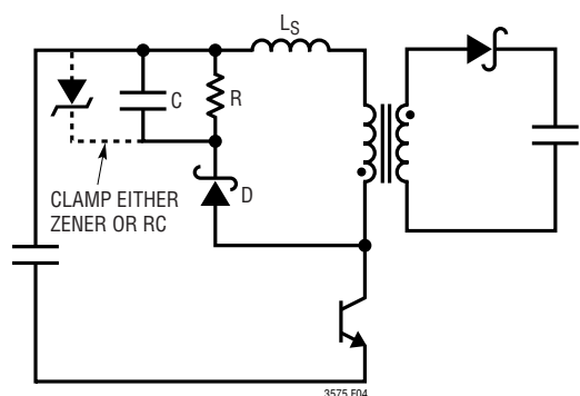
Figure 4. Snubber Clamping
