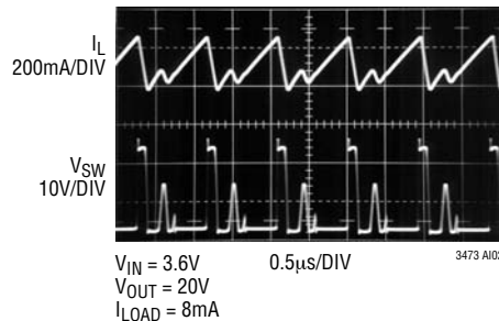
Switching Waveforms
