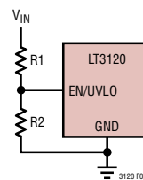
Figure 8. Setting the Input UVLO and Hysteresis
