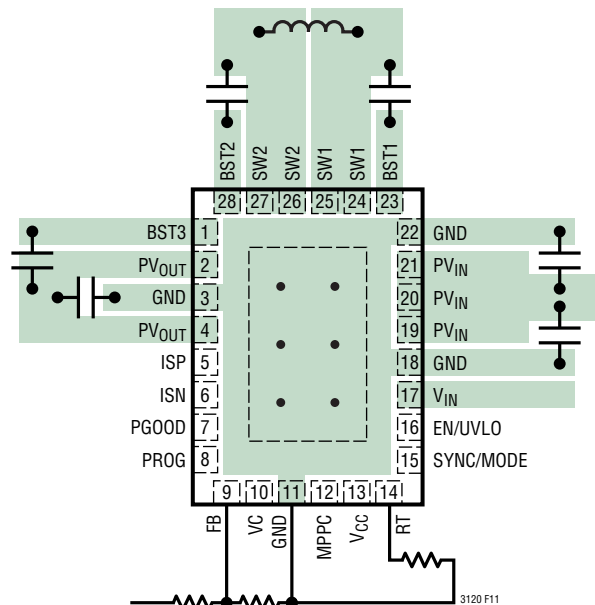
Figure 11. PCB Layout
