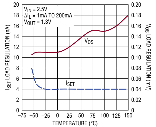
Load Regulation
