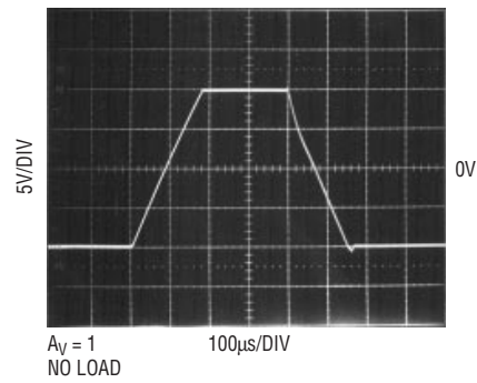
Large-Signal Transient Response V_S = \pm 15V
