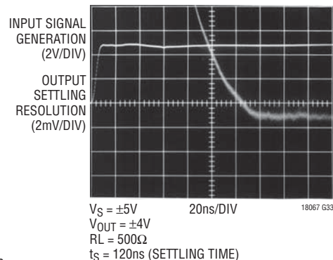
0.01% Settling Time
