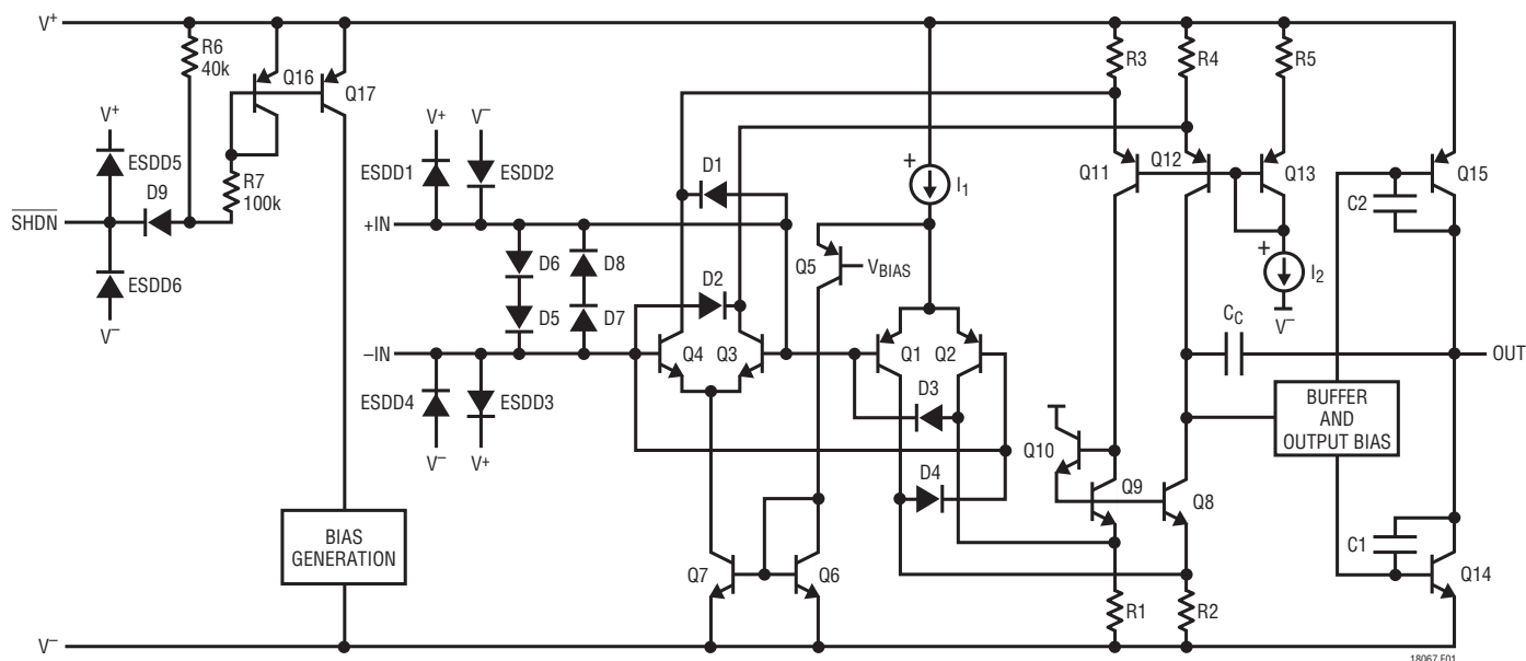
Figure 1. LT1806 Simplified Schematic Diagram
