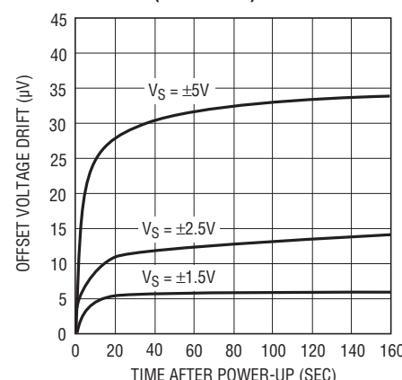
Warm-Up Drift vs Time (LT1806S8)
