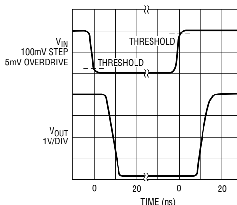
Response Time
