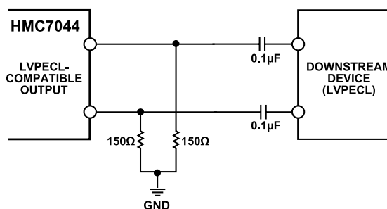
Figure 34. AC-Coupled LVPECL Output Driver
