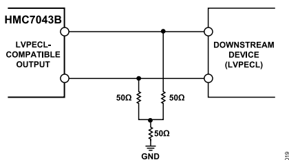
Figure 21. DC-Coupled LVPECL Output Driver
