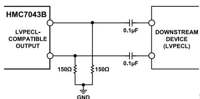
Figure 18. AC-Coupled LVPECL Output Driver
