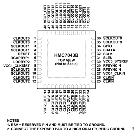
Figure 2. Pin Configuration
