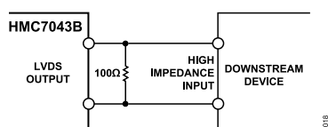
Figure 20. DC-Coupled LVDS Output Driver
