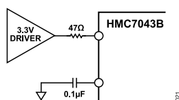
Figure 23. CLKIN, RFSYNCIN Input Single-Ended Mode
