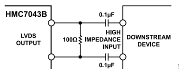
Figure 15. AC-Coupled LVDS Output Driver
