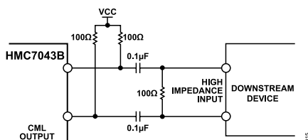
Figure 16. AC-Coupled CML (Configured High-Z) Output Driver
