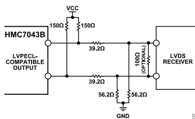
Figure 24. Level Translation for LVDS N-Pulse Operation (Place 100 Ω Termination Resistor If Receiver Does Not Have It)
