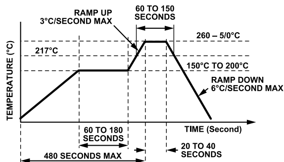
Figure 33. Pb-Free Reflow Solder Profile
