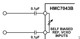
Figure 19. CLKIN/CLKIN, RFSYNCIN Input Differential Mode
