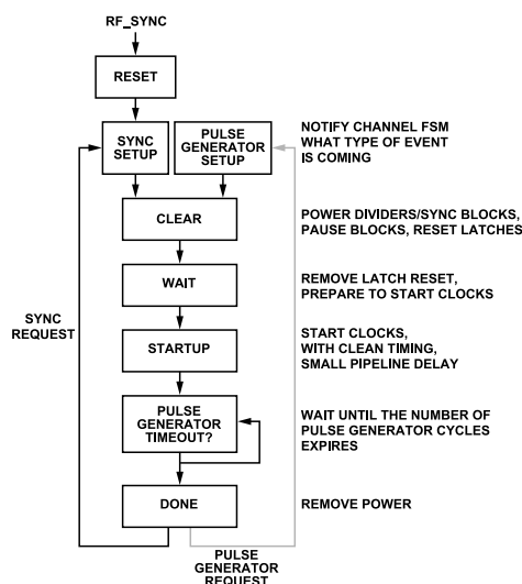
Figure 28. Synchronization FSM Flowchart
