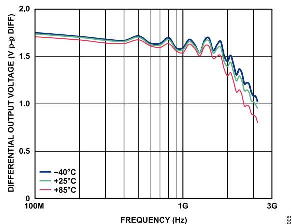
Figure 7. LVPECL Differential Output Power vs. Frequency over Various Temperatures
