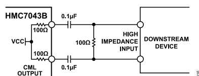
Figure 17. AC-Coupled CML (Internal) Output Driver
