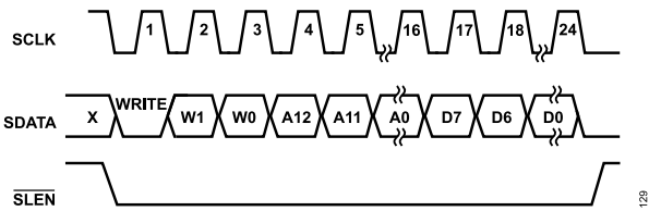
Figure 32. SPI Timing Diagram, Write Operation
