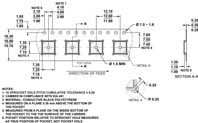
Figure 34. LFCSP Tape and Reel Outline Dimensions Shown in Millimeters
