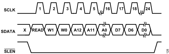
Figure 31. SPI Timing Diagram, Read Operation
