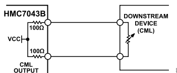
Figure 22. DC-Coupled CML (Internal) Output Driver
