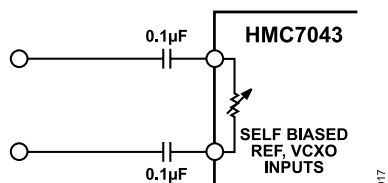
Figure 19. CLKIN/CLKIN, RFSYNCIN Input Differential Mode
