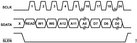
Figure 32. SPI Timing Diagram, Read Operation
