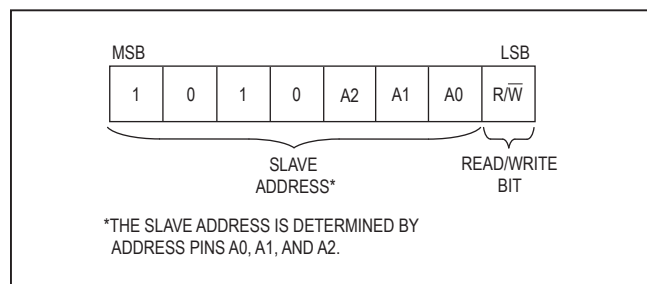
Figure 1. DS4520 Slave Address Byte
