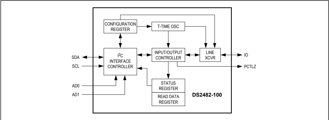
Figure 1. Block Diagram
