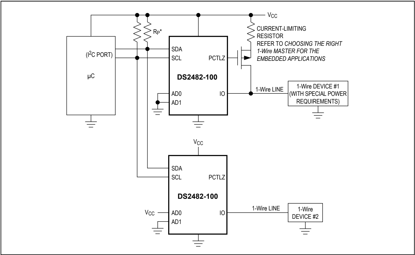
Figure 10. Application Schematic
