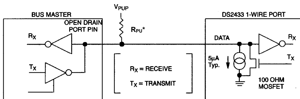
Figure 8. HARDWARE CONFIGURATION
