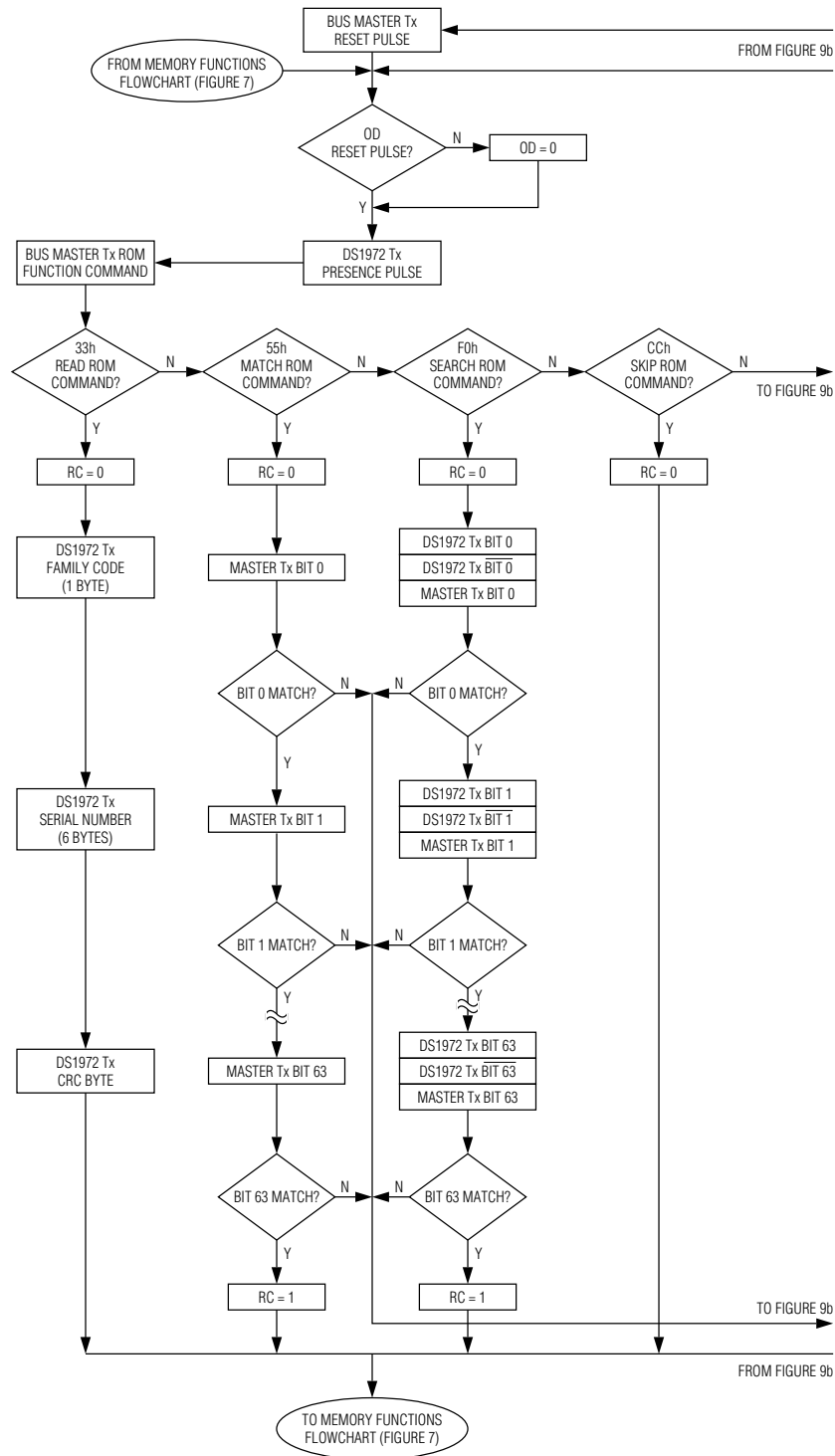
Figure 9a. ROM Functions Flowchart
