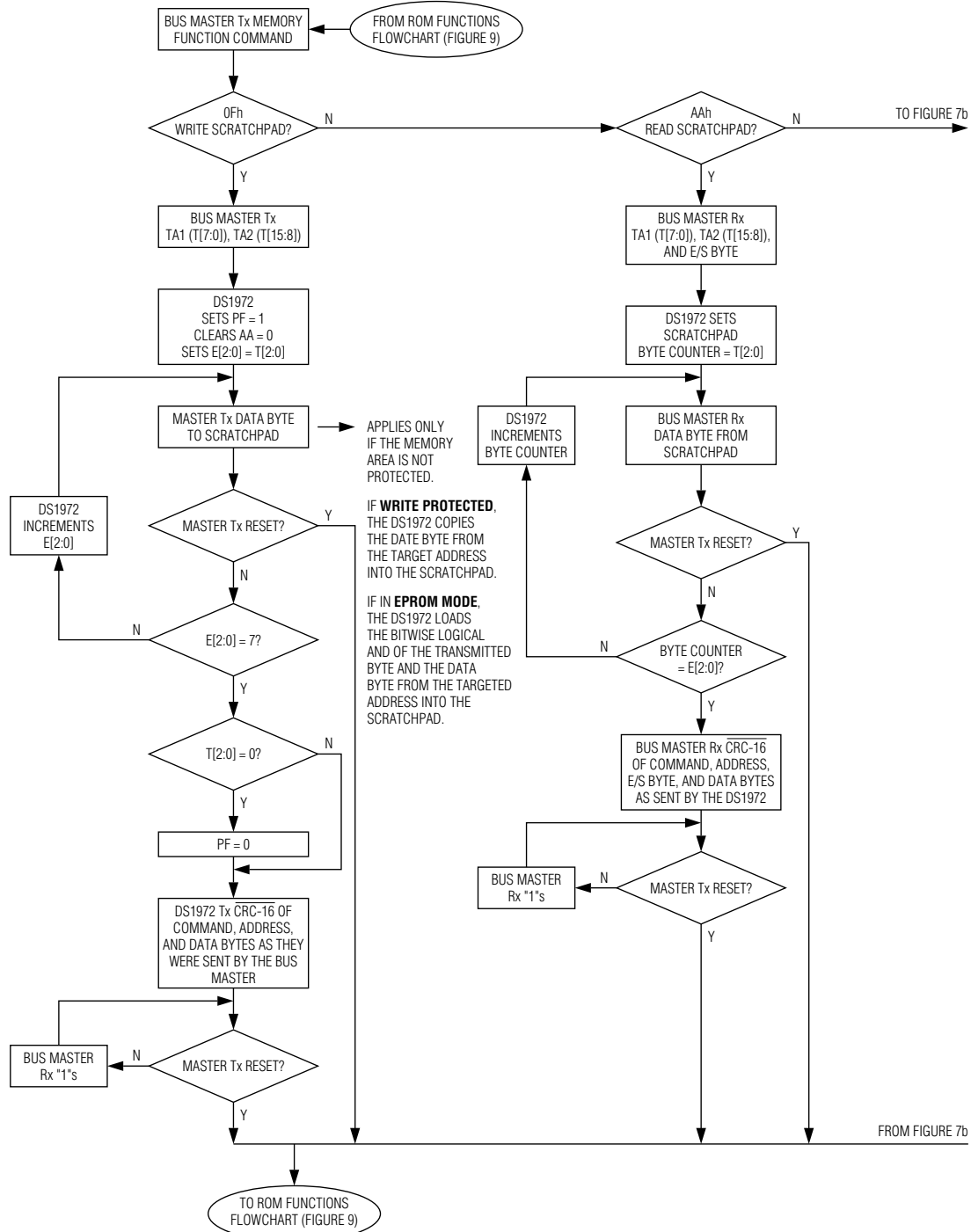
Figure 7a. Memory Function Flowchart
