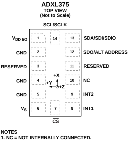
Figure 3. Pin Configuration
