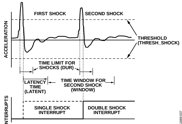
Figure 33. Shock Interrupt Function with Valid Single and Double Shocks
