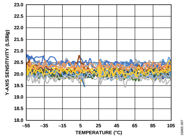
Figure 7. Y-Axis Sensitivity vs. Temperature, 15 Devices Soldered to PCB, V_S = 2.5 V
