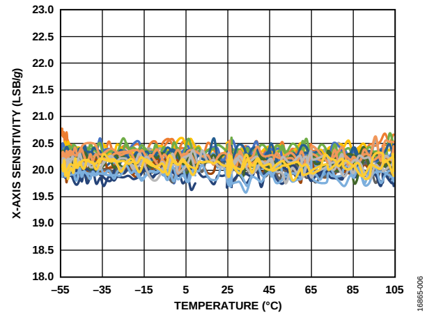
Figure 6. X-Axis Sensitivity vs. Temperature, 15 Devices Soldered to PCB, V_S = 2.5 V
