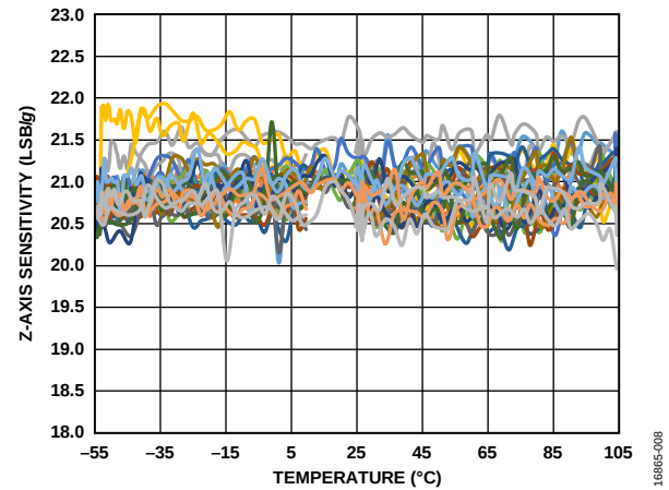
Figure 8. Z-Axis Sensitivity vs. Temperature, 15 Devices Soldered to PCB, V_S = 2.5 V
