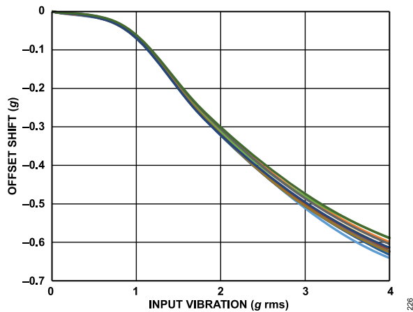
Figure 27. ADXL354 VRE, Y-Axis Offset from +1 g, \pm 2 g Range, Y-Axis Orientation = +1 g
