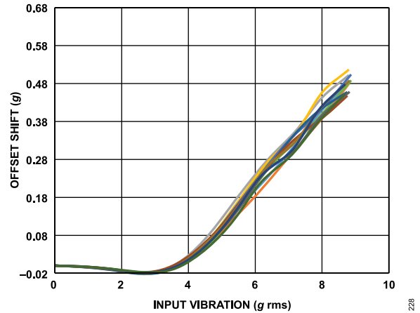
Figure 29. ADXL354 VRE, X-Axis Offset from -1 g, \pm 8 g Range, X-Axis Orientation = -1 g
