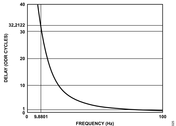
Figure 66. High-Pass Filter Delay Response for a 4 kHz ODR and an HPF_CORNER Setting of 001 (Register 0x28, Bits[6:4])
