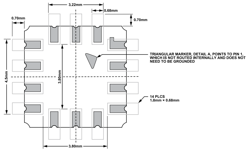
Figure 80. PCB Footprint Pattern and Dimensions in Millimeters
