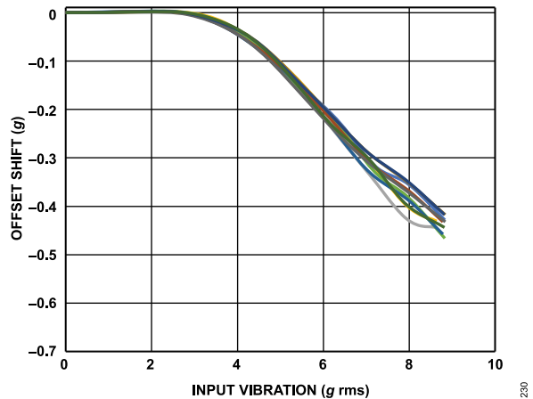
Figure 31. ADXL354 VRE, Z-Axis Offset from +1 g, \pm 8 g Range, Z-Axis Orientation = +1 g
