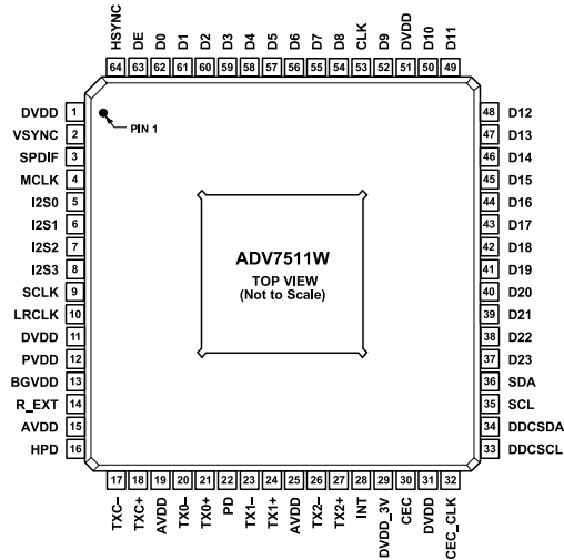
Figure 2. Pin Configuration
