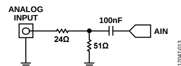
Figure 11. Typical Single-Ended Input Voltage Divider Network
