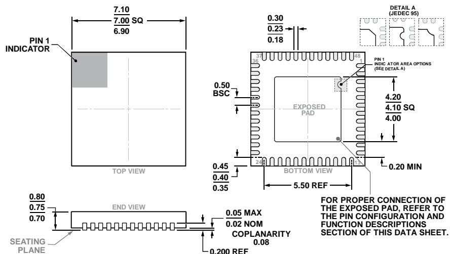
Figure 4. 48-Lead Lead Frame Chip Scale Package [LF CSP] 7 mm x 7 mm Body and 0.75 mm Package Height (CP-48-5)
