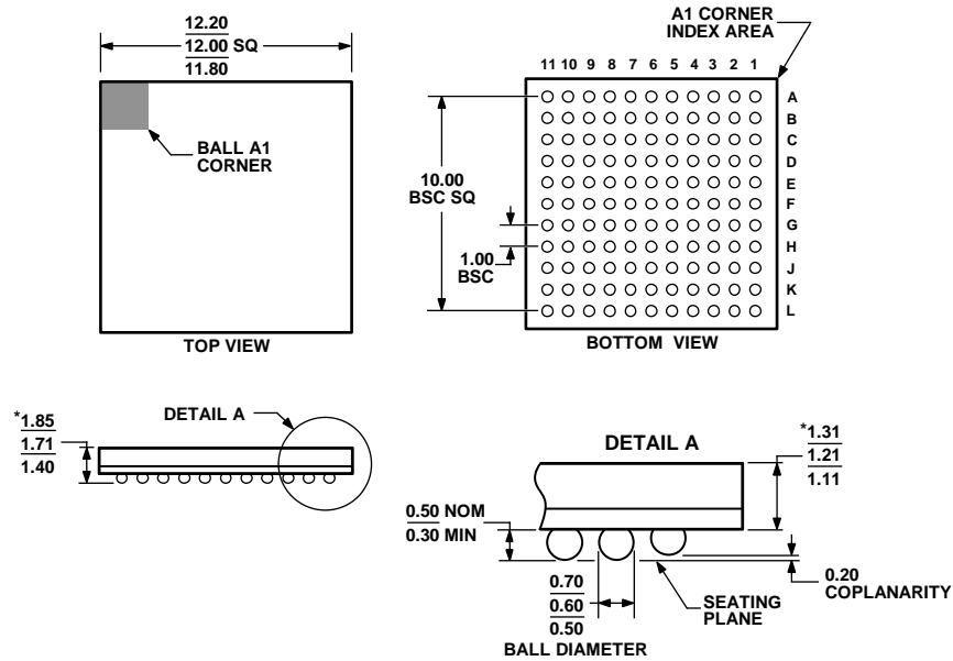
Figure 40. 121-Ball Chip Scale Package Ball Grid Array [CSP_BGA] (BC-121-1) Dimensions shown in millimeters
