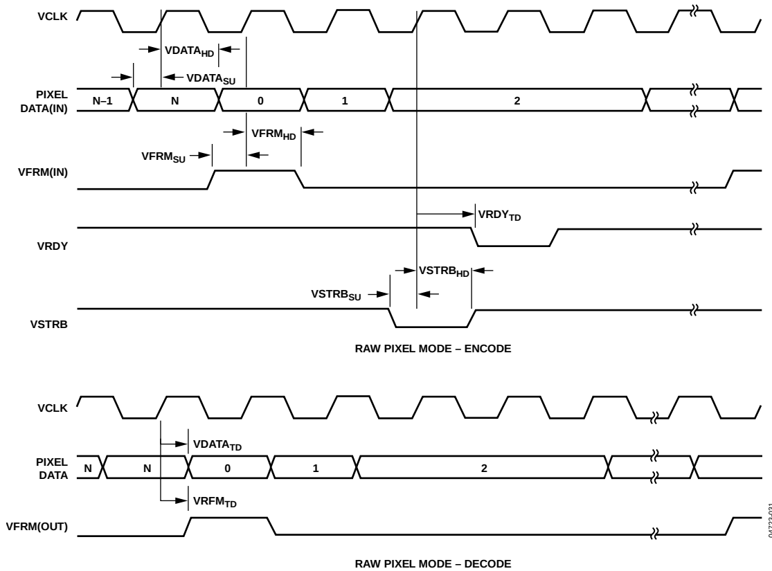
Figure 22. Raw Pixel Mode Timing
