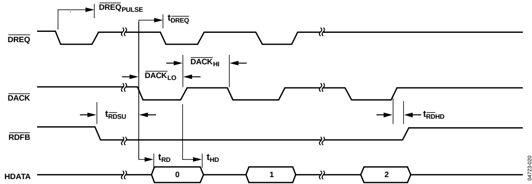
Figure 11. Fly-By DMA Mode—Single Read Cycle ( \overline{DREQ} Pulse Width Is Programmable)
