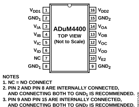
Figure 5. ADuM4400 Pin Configuration
