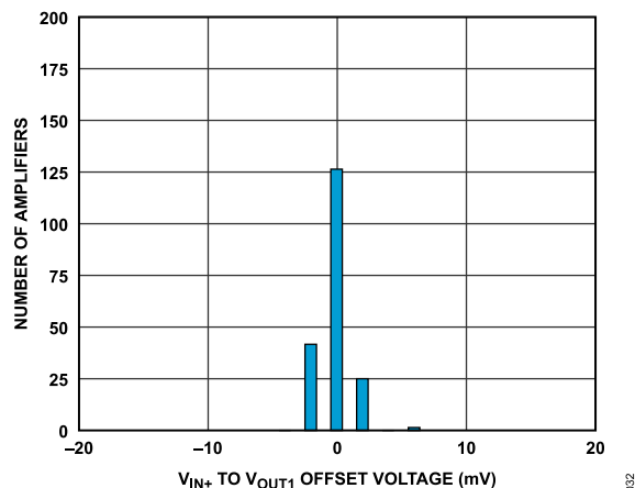
Figure 32. V_{IN+} to V_{OUT1} Offset-Voltage Distribution at 125°C
