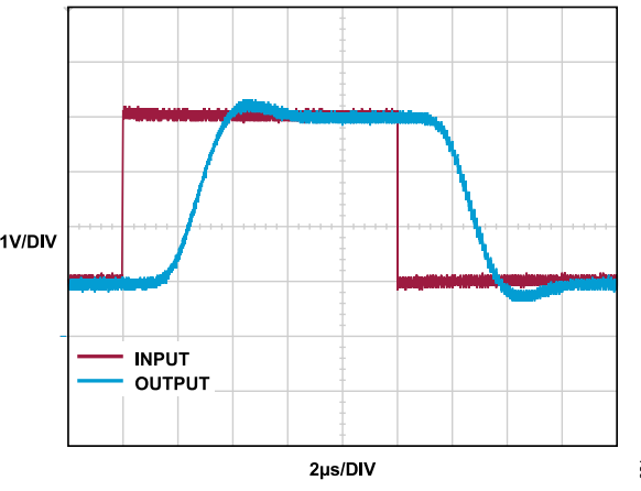
Figure 21. Output Square-Wave Response
