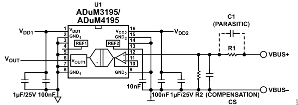
Figure 37. DC Bus Voltage Monitoring Using ADuM3195/ADuM4195
