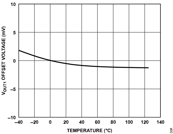
Figure 8. V_{OUT1} Offset Voltage vs. Temperature
