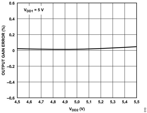
Figure 10. Output Gain Error vs. V_{DD2}
