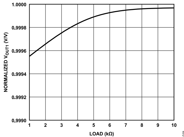
Figure 19. Normalized V_{\text{OUT1}} vs. Load
