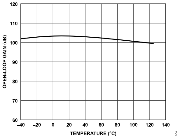
Figure 6. Op Amp Open-Loop Gain vs. Temperature
