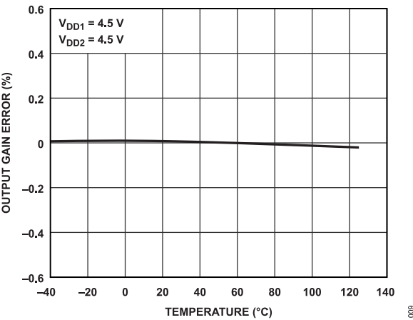
Figure 9. Output Gain Error vs. Temperature
