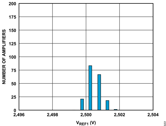
Figure 22. V_{\text{REF1}} Distribution at 25 ^{\circ}\text{C}
