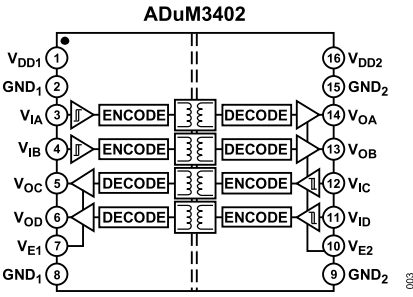
Figure 3. ADuM3402 Functional Block Diagram
