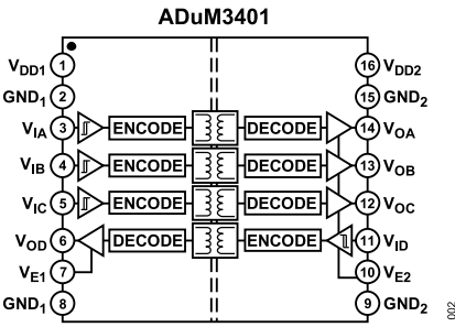
Figure 2. ADuM3401 Functional Block Diagram
