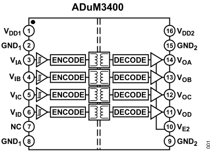
Figure 1. ADuM3400 Functional Block Diagram
