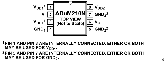
Figure 3. Pin Configuration
