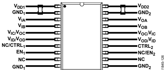
Figure 30. Recommended Printed Circuit Board Layout, SSOP
