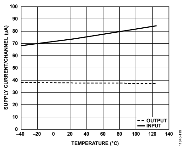
Figure 23. Typical Input and Output Supply Current per Channel vs. Temperature for V_{DDx} = 2.5 V, Data Rate = 1000 kbps
