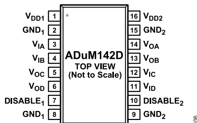
Figure 11. ADuM142D Pin Configuration
