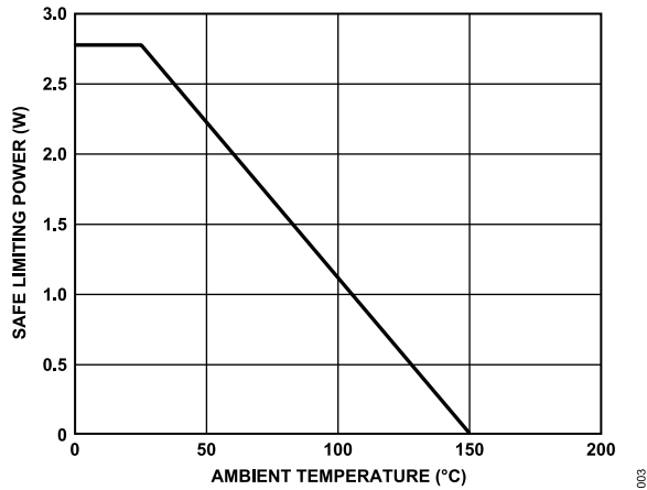
Figure 5. Thermal Derating Curve for RW-16 Wide Body [SOIC_W] Package, Dependence of Safety Limiting Values with Ambient Temperature per DIN EN IEC 60747-17 (VDE 0884-17)
