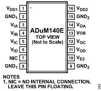
Figure 8. ADuM140E Pin Configuration
