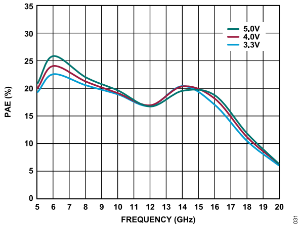
Figure 31. Power Added Efficiency (PAE) vs. Frequency for Various V_{DD\_PA} , Transmit State, Path = TX_IN to ANT, I_{DQ\_PA} = 220\text{ mA} , Receive State Off, PAE Measured at P_{SAT}
