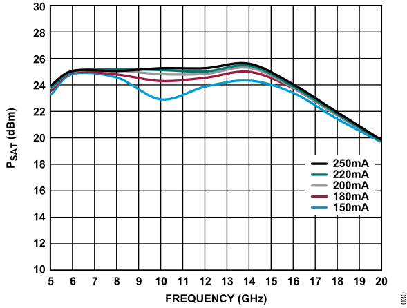
Figure 30. P_{SAT} vs. Frequency for Various I_{DQ\_PA} , Transmit State, Path = TX_IN to ANT, V_{DD\_PA} = 5\text{ V} , Receive State Off
