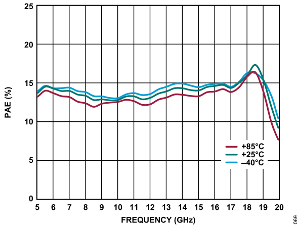
Figure 69. PAE vs. Frequency for Various Temperatures, Receive State, Path = ANT to RX_OUT, Self Biased Mode, V_{DD\_LNA} = 3.3\text{ V} , V_{GG\_LNA} = 0\text{ V} , Transmit State Off, PAE Measured at P_{SAT}
