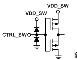
Figure 5. CTRL_SW and VDD_SW Interface Schematic
