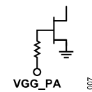
Figure 7. VGG_PA Interface Schematic
