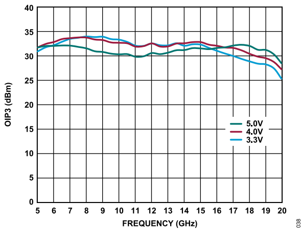
Figure 38. OIP3 vs. Frequency for Various V_{DD\_PA} , P_{OUT}/\text{Tone} = 8\text{ dBm} , Transmit State, Path = TX_IN to ANT, I_{DQ\_PA} = 220\text{ mA} , Receive State Off
