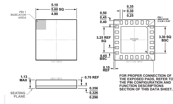
Figure 92. 24-Terminal Land Grid Array [LGA] (CC-24-8)
