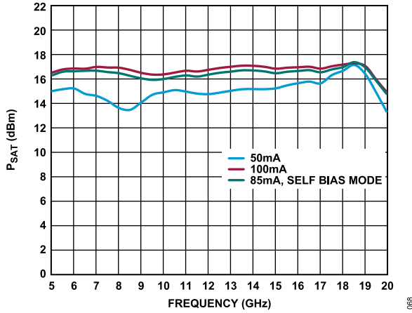
Figure 68. P_{SAT} vs. Frequency for Various I_{DD\_LNA} , Receive State, Path = ANT to RX_OUT, Self Biased Mode, V_{DD\_LNA} = 3.3\text{ V} , Controlled V_{GG\_LNA} , Transmit State Off
