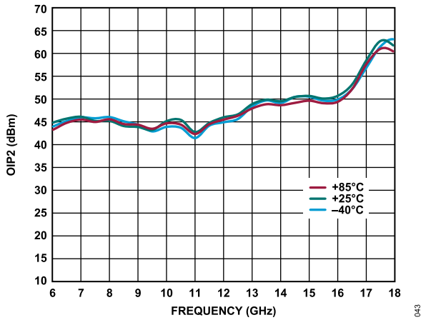
Figure 43. Output Second-Order Intercept (OIP2) vs. Frequency for Various Temperatures, P_{OUT}/Tone = 8\text{ dBm} , Transmit State, Path = TX_IN to ANT, V_{DD\_PA} = 5\text{ V} , I_{DQ\_PA} = 220\text{ mA} , Receive State Off
