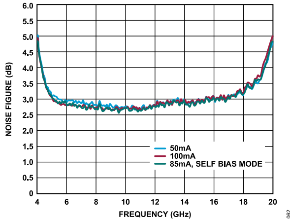
Figure 62. Noise Figure vs. Frequency for Various I_{DQ\_LNA} , Receive State, Path = ANT to RX_OUT, Self Biased Mode, V_{DD\_LNA} = 3.3\text{ V} , Controlled V_{GG\_LNA} , Transmit State Off
