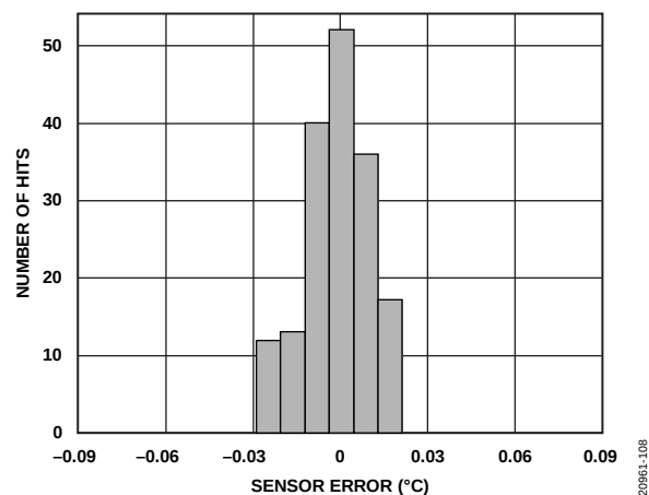
Figure 8. Histogram Distribution of Factory Calibration Error at 38°C for 170 Devices, V_{DD} = 3\text{ V}
