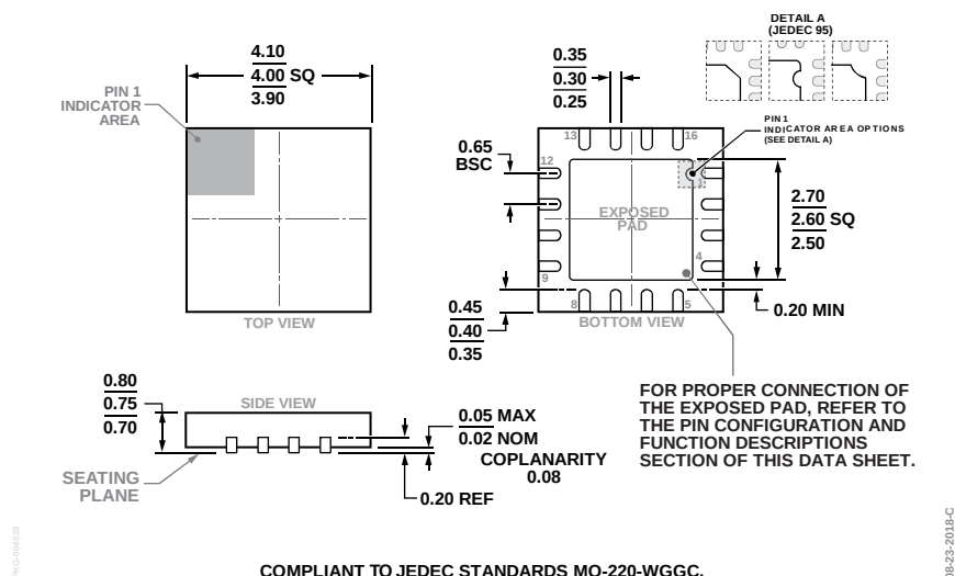
Figure 23. 16-Lead Lead Frame Chip Scale Package [LFCSP] 4 mm × 4 mm Body and 0.75 mm Package Height (CP-16-17)
