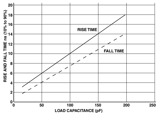
Figure 55. Typical Output Delay or Hold for Driver C at V_{DDEXT} Max
