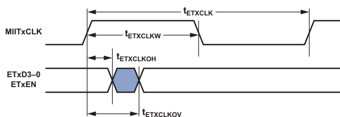
Figure 30. 10/100 Ethernet MAC Controller Timing: MII Transmit Signal
